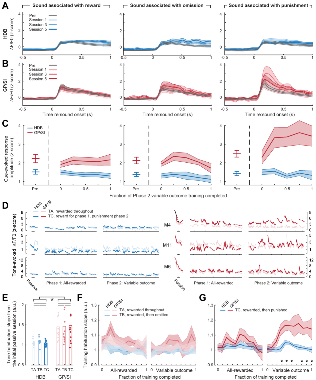
Figure 7. Enhanced BFCN responses to punishment-predicting cues in GP/Sl, not HDB. (A-B) Mean \pm SEM tone-evoked GCaMP activity in HDB (N=11, A) and GP/Sl (B) for the tone frequency associated with reward (left column), reward omission (middle column), and
