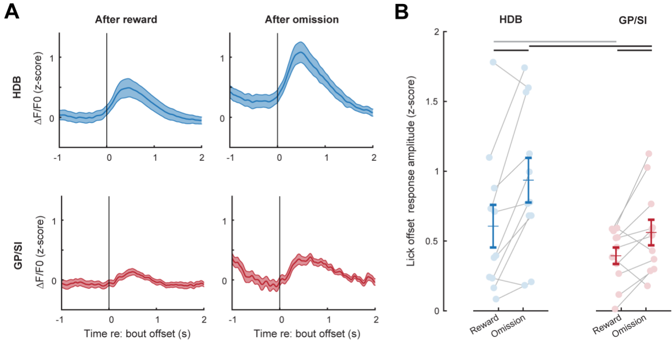
Figure 6 – figure supplement 1. Basal forebrain responses on omission trials reflect reinforcement prediction error, not a motor-related signal.
